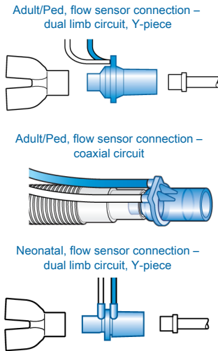
Figure 3-7. Connecting the flow sensor to the Y-piece or circuit
