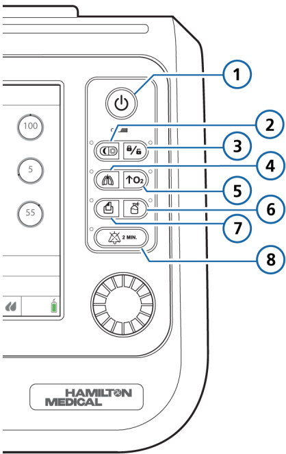
Figure 10-2. Function keys
