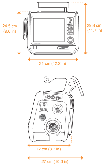
Figure 15-1. HAMILTON-T1 dimensions
