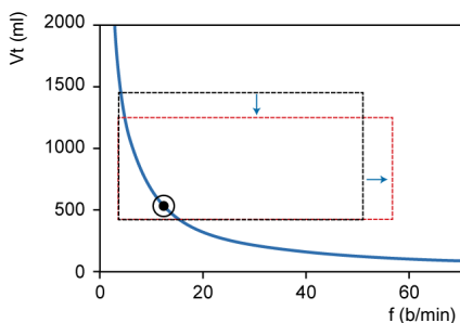
Figure 7-26. Lung-protective limits
