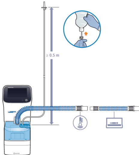
Incubator setup
